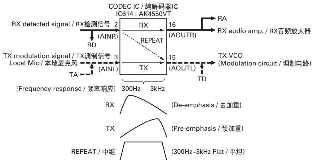
Fig. 9 An audio signal course and the frequency characteristic / 图9 音频信号路线和频率特性
