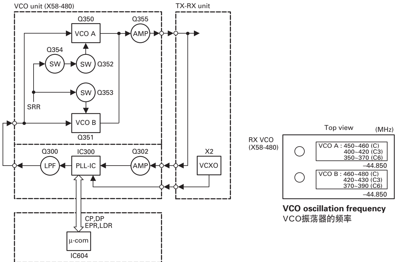
Fig. 5 Receiver PLL / 图5 接收机PLL
